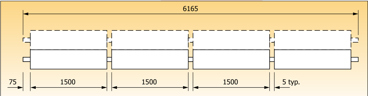
M1 and M2 strip - nominal length 6.0m
