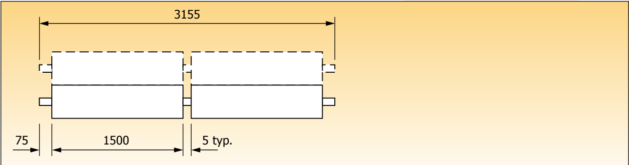
M1 and M2 strip - nominal length 3.0m
