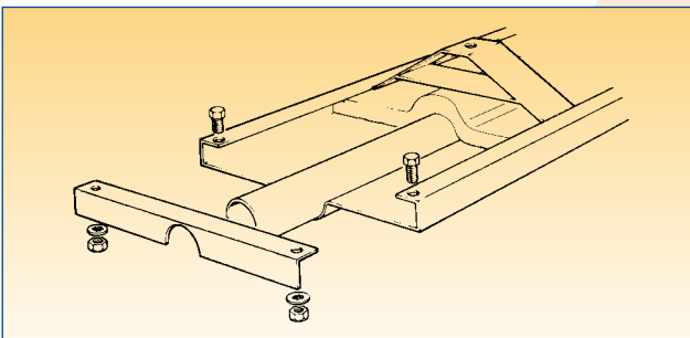
EC1 - End closer for M1 Dunham Strip
